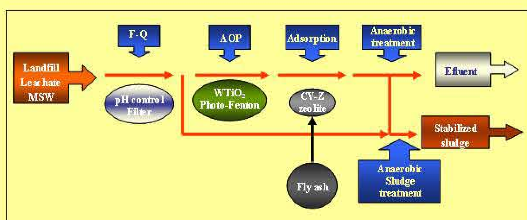
Figure 1. Schematic representation of the experimental process.
