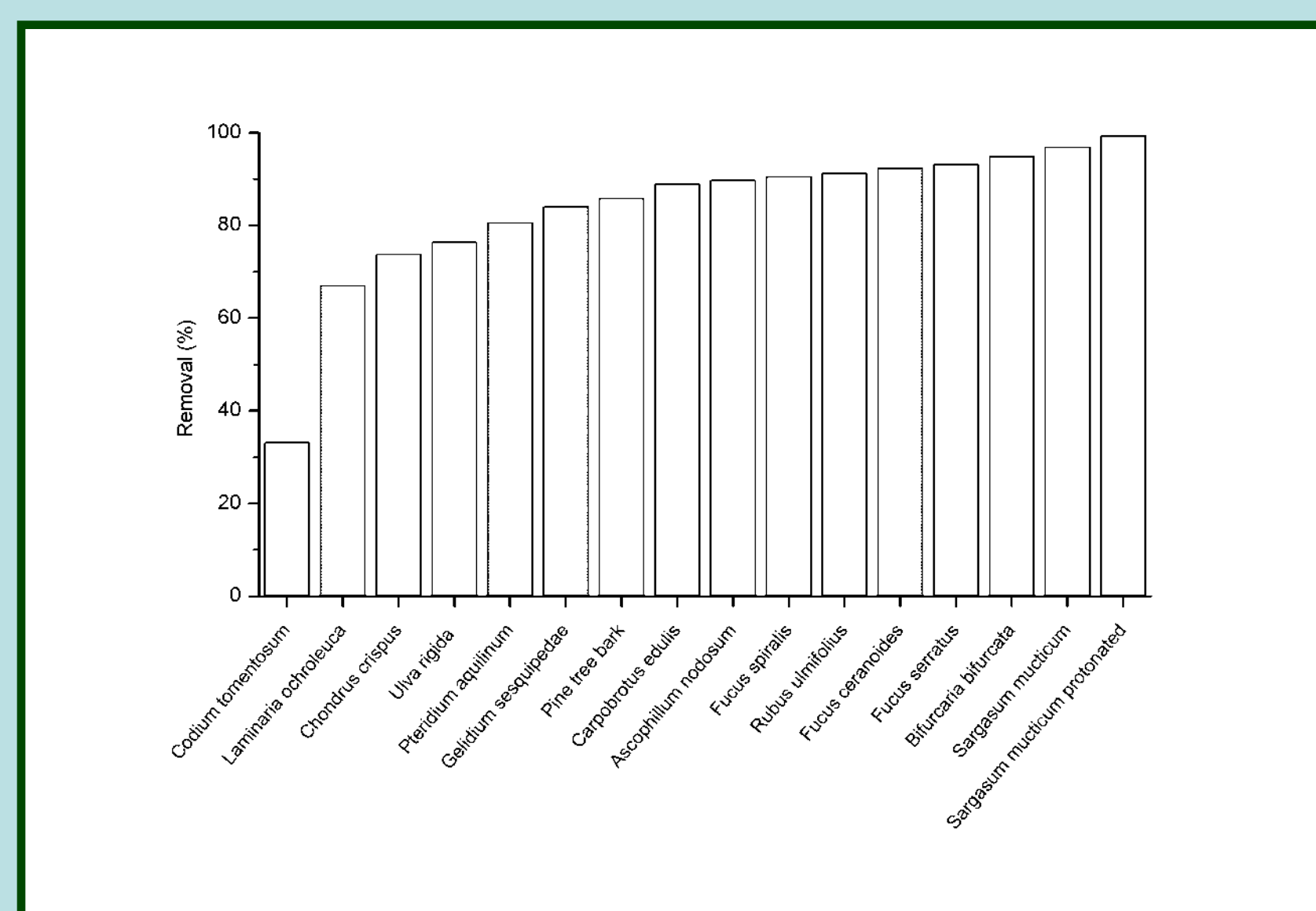
Figure 2. Screening of mercury sorption onto different natural materials. Initial mercury concentration of 0.5 mmol/L. pH interval 4.5-5. Sorbent dose 2.5 g/L. Mercury removal values after 24 h of equilibrium.
