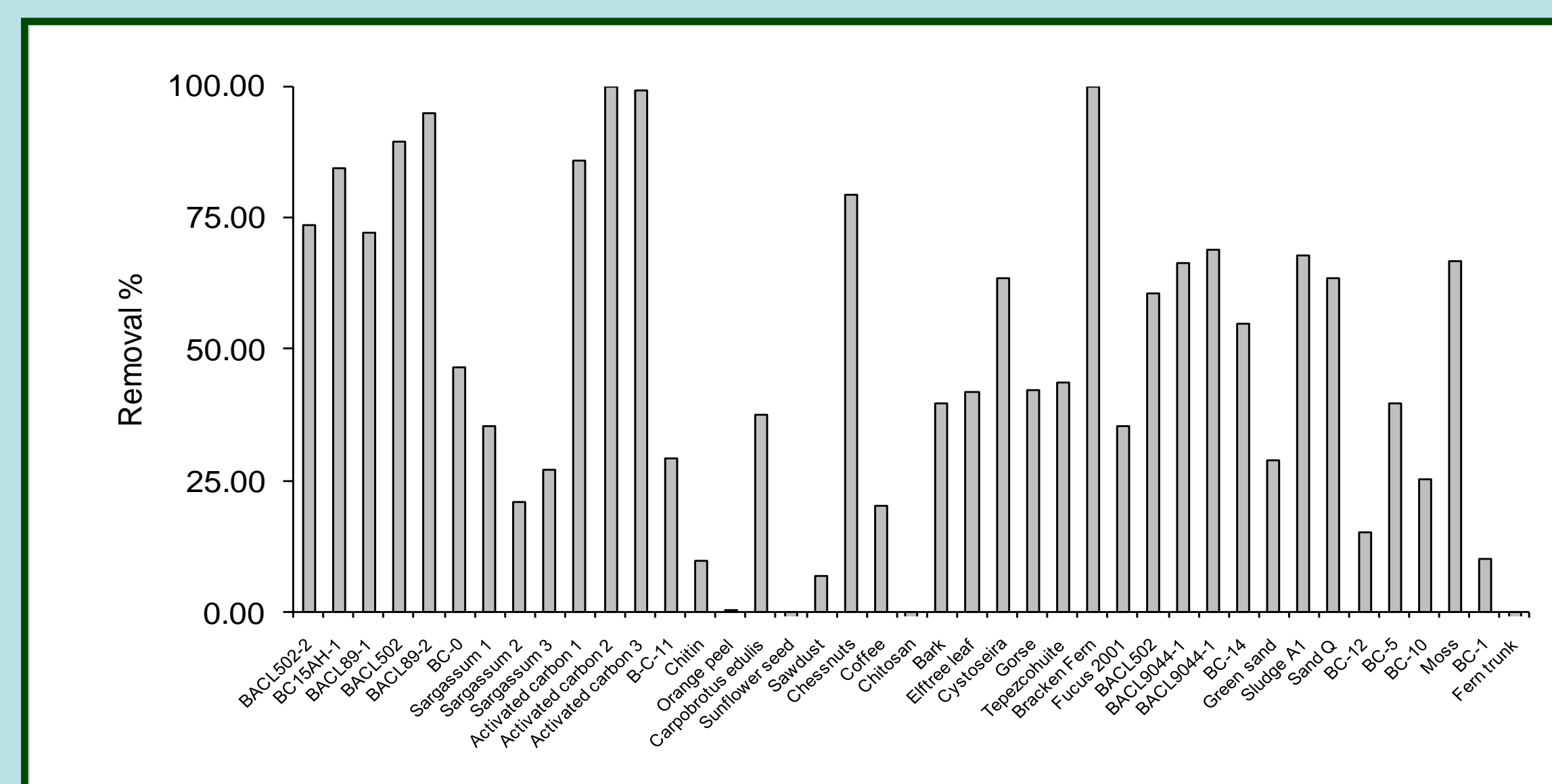
Figure 3. Screening of flumequine sorption onto different natural materials. Initial flumequine concentration 50 µg/L. Sorbent dose 2.5 g/L. Natural pH.
