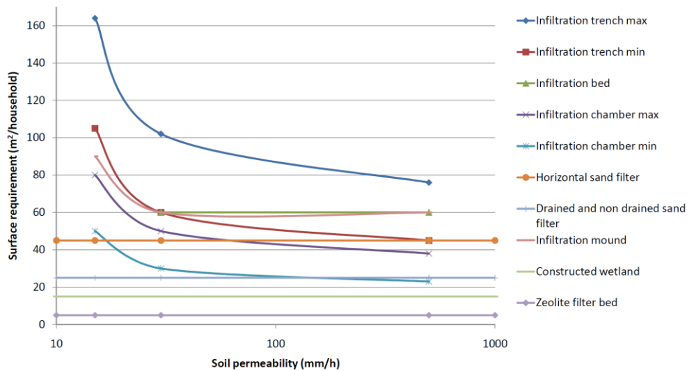
Figure 1. Surface requirement based on soil permeability and treatment system (Collado, 2006)
