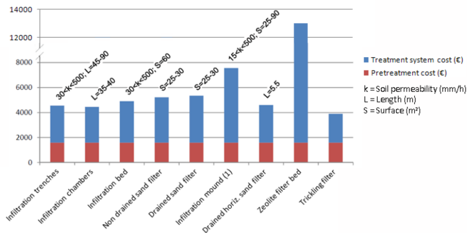
Figure 2. Treatment system costs for a 4 person household unit. (1) Including pumping station cost of 1,450 €
